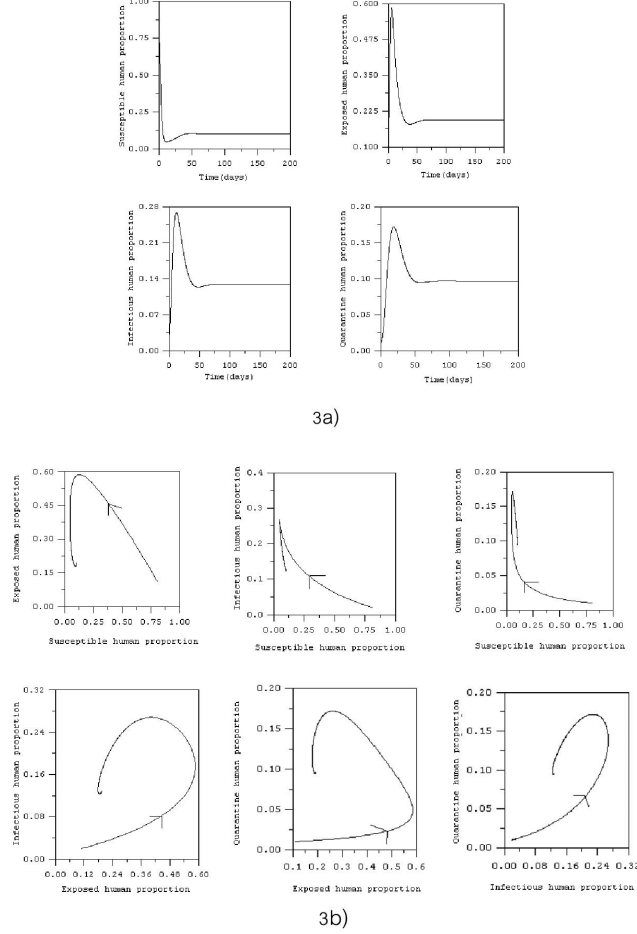
Figure 3: Behaviors of our model for R_0 > 1 . The values of parameters are c = \frac{1}{30} per day, \mu_h = \frac{1}{365 \times 65} per day, \varepsilon = \frac{1}{10} per day, b = \frac{1}{40} per day, \theta = \frac{1}{6} per day, \alpha = \frac{1}{30} per day, \beta = \frac{1}{8} per day, \gamma = 0.8 and R_0 = 10 . 3a) Time series solutions of susceptible, exposed, infectious and quarantine human proportions, respectively. 3b) The trajectories of solutions projected onto the (S,E) , (S,I) , (S,Q) , (E,I) , (E,Q) and (I,Q) planes. The fractions of populations (S^*, E^*, I^*, Q^*) approach to the endemic disease steady state (0.100043, 0.193052, 0.128665, 0.0964747) .
