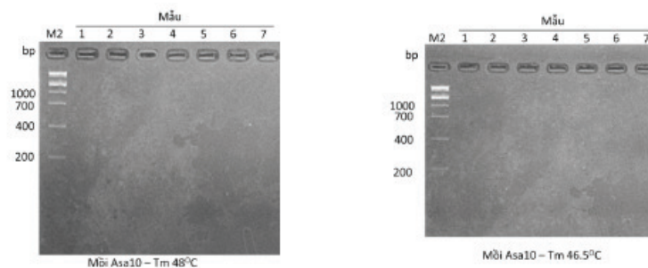
Fig 3.5 Electrophoresis graph of the PCR products from seven garlic samples with primer Asa10. M2: ZipRuler Express DNA Ladder 2; arrows indicate the target bands.
