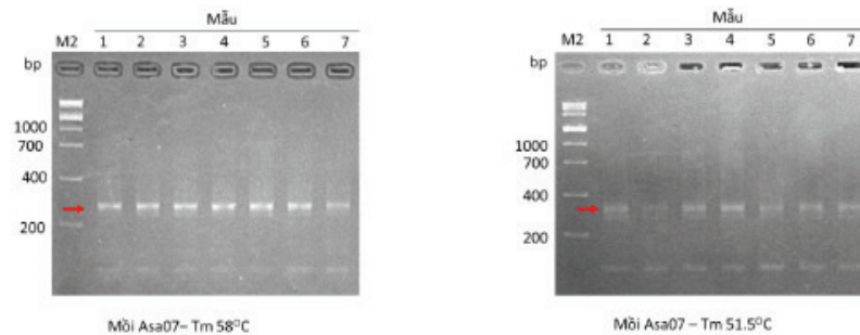
Fig 3.3 Electrophoresis graph of the PCR products from seven garlic samples with primer Asa07. M2: ZipRuler Express DNA Ladder 2; arrows indicate the target bands.
