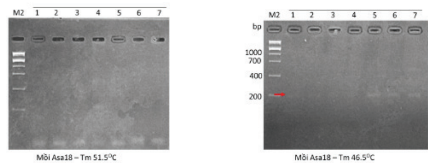
Fig 3.9 Electrophoresis graph of the PCR products from seven garlic samples with primer Asa18. M2: ZipRuler Express DNA Ladder 2; arrows indicate the target bands.
