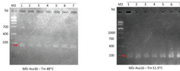
Fig 3.7 Electrophoresis graph of the PCR products from seven garlic samples with primer Asa16. M2: ZipRuler Express DNA Ladder 2; arrows indicate the target bands.
