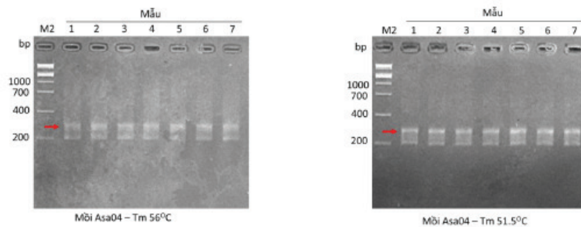
Fig 3.1 Electrophoresis graph of the PCR products from seven garlic samples with primer Asa04. M2: ZipRuler Express DNA Ladder 2; arrows indicate the target bands.
