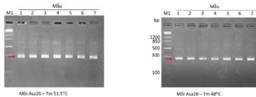
Fig 3.10 Electrophoresis graph of the PCR products from seven garlic samples with primer Asa20. M2: ZipRuler Express DNA Ladder 2; arrows indicate the target bands.
