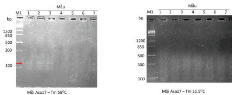
Fig 3.8 Electrophoresis graph of the PCR products from seven garlic samples with primer Asa17. M2: ZipRuler Express DNA Ladder 2; arrows indicate the target bands.
